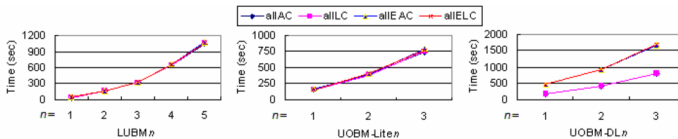
Figure 2: The execution time of the preprocess phase
