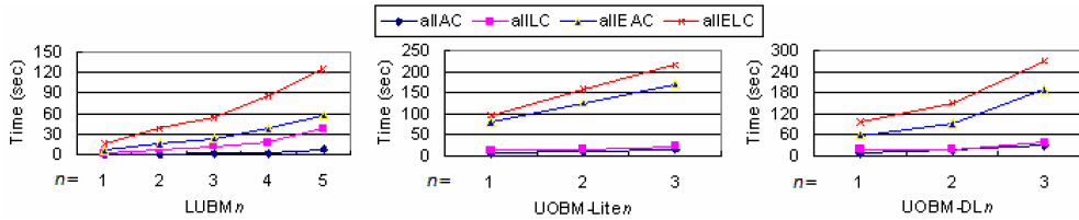
Figure 4: The average execution time for computing abductive solutions for a successful observation
