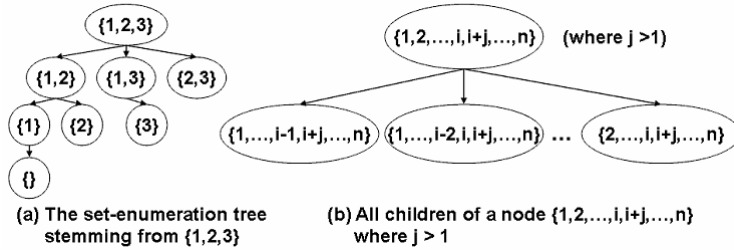
Figure 1: Illustrations for set-enumeration trees
