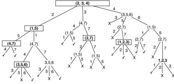
Fig. 3. Computing all justifications using Reiter's Hitting Set Tree Algorithm from [10].
