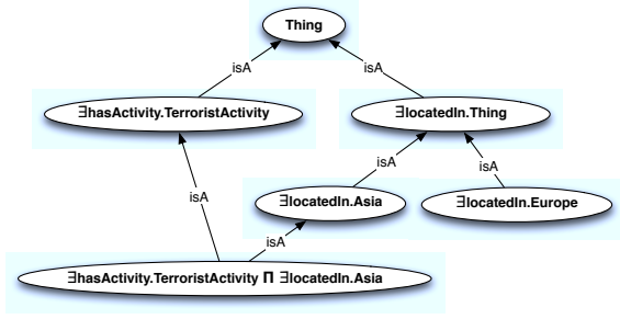
Fig. 2. Context hierarchy
